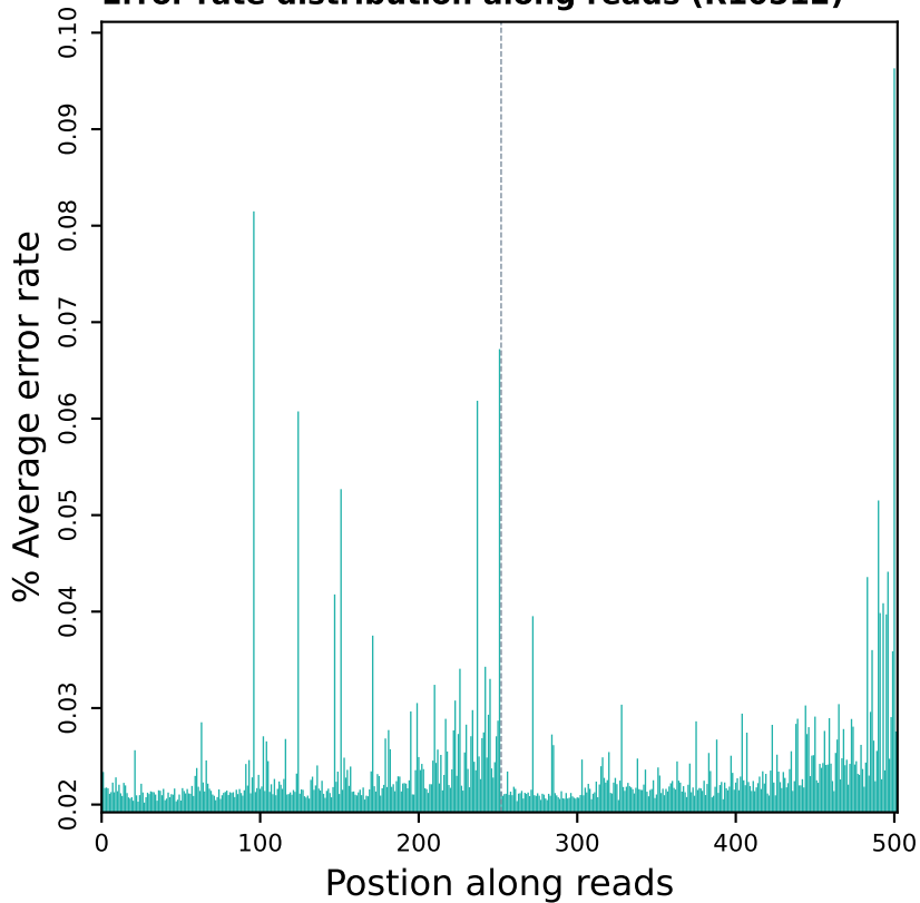
Error rate distribution along reads (R10512)
